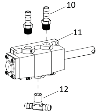
Air Motor Pedal Valve Assembly
