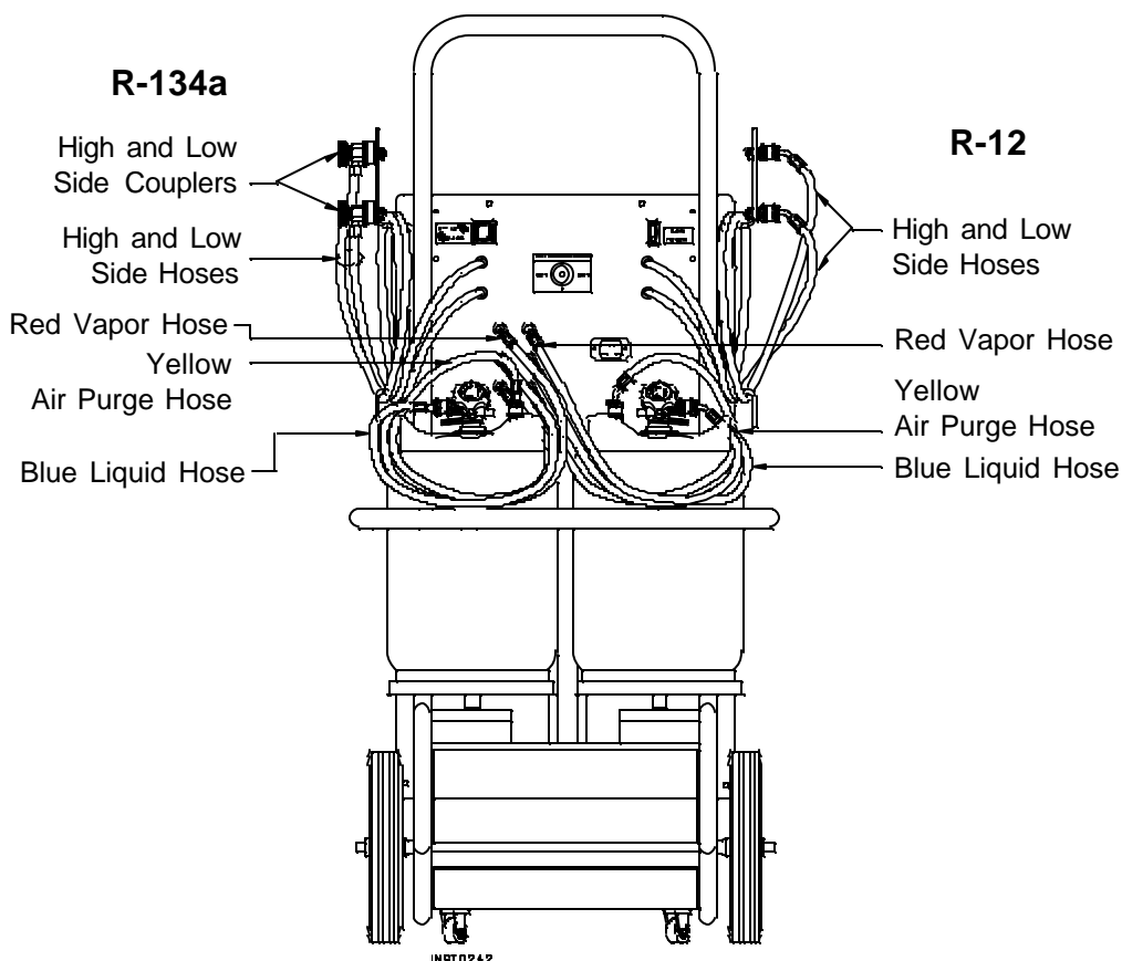
Diagram of Hose Connections
