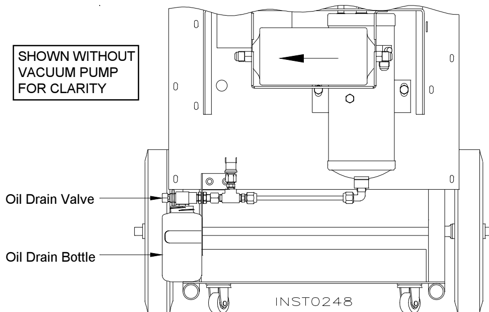
Diagram of Oil Drain Valve and Bottle
