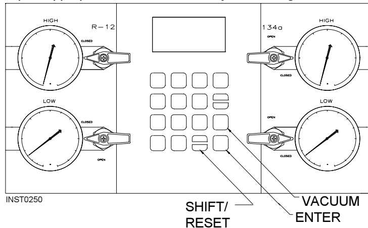
Diagram of Control Panel For R-12 Or R-134a
