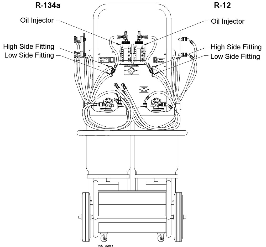
Diagram of Oil Injection System
