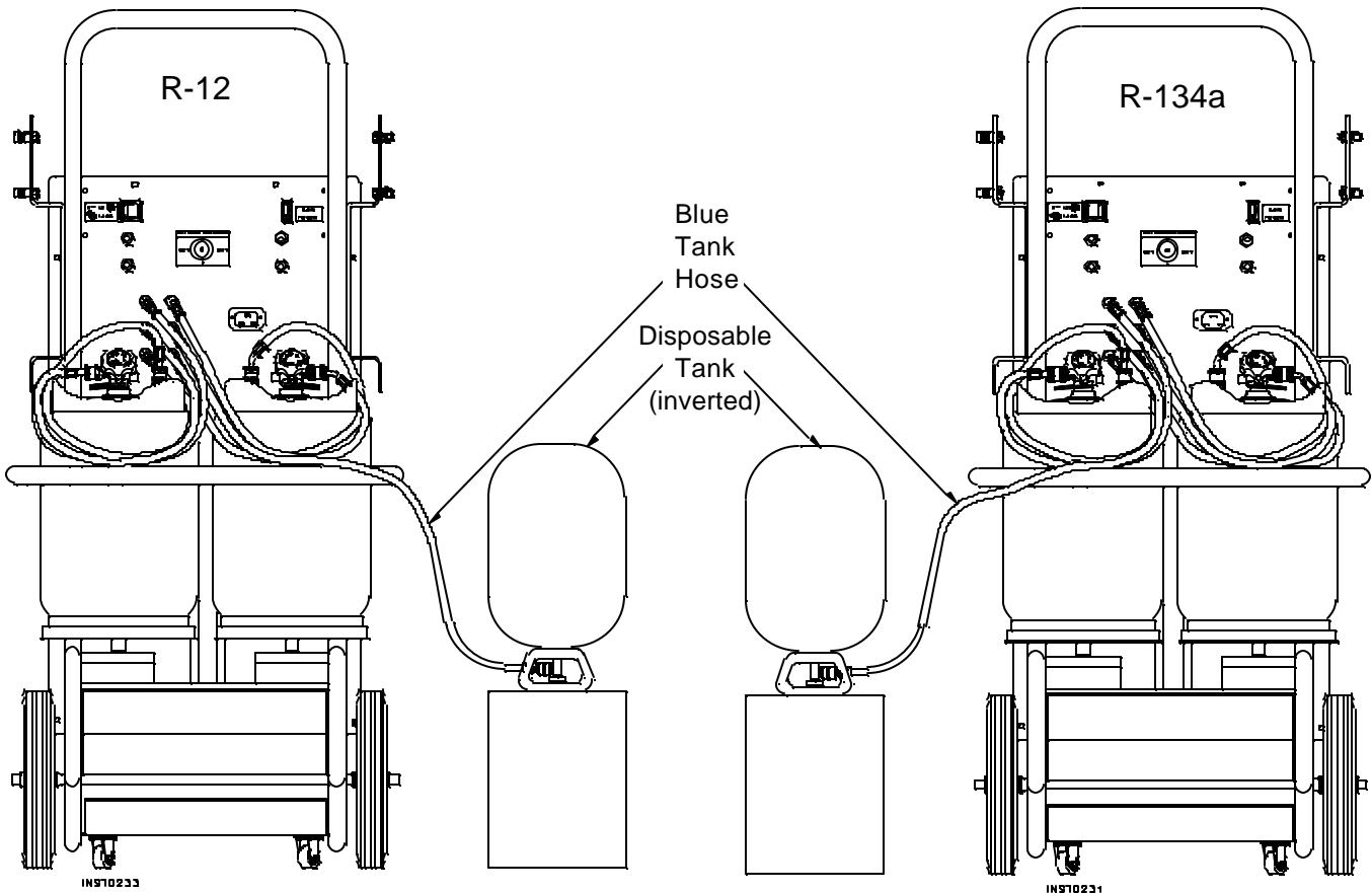
Diagram of Disposable Tank Connections When Adding Refrigerant
