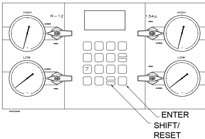
Diagram of Control Panel For R-12 Or R-134a
