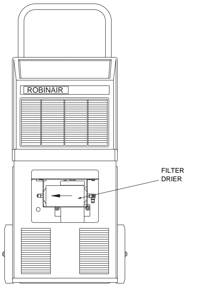
Diagram of Filter-Drier Location
