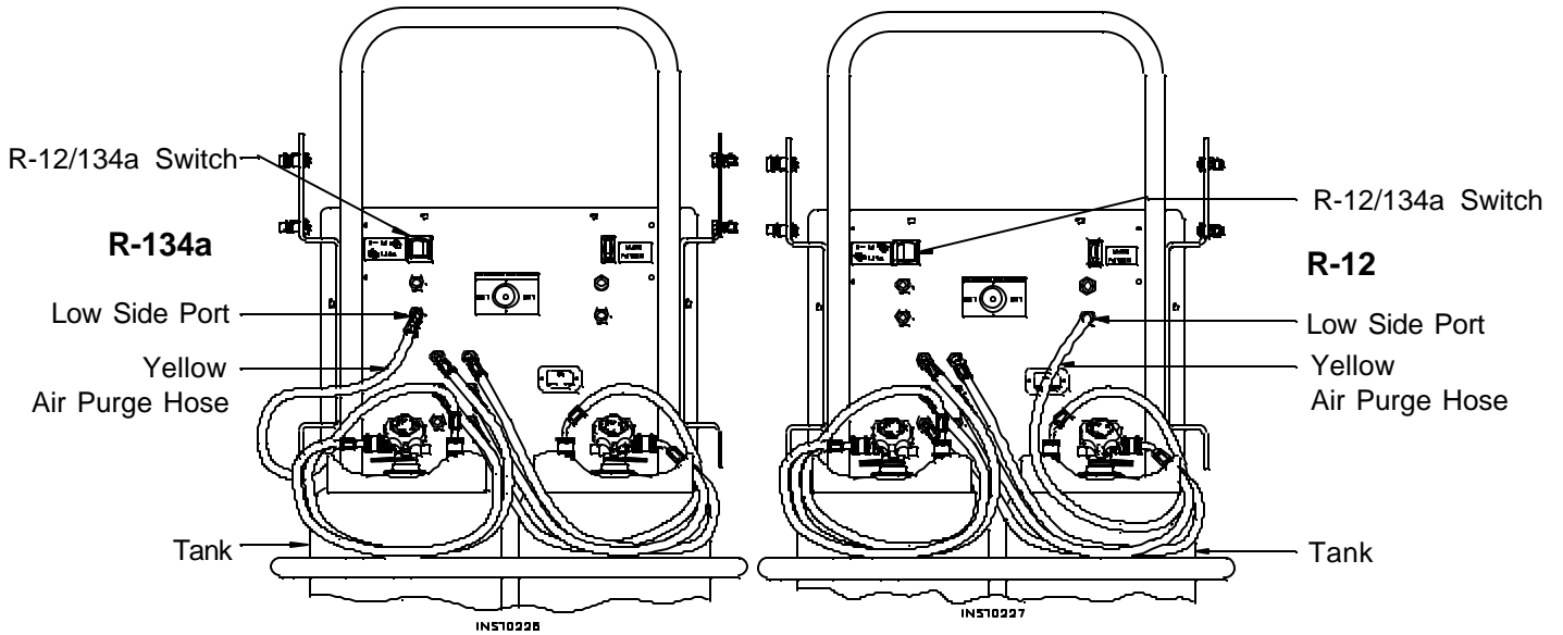
Diagram of Tank Connections During Evacuation
