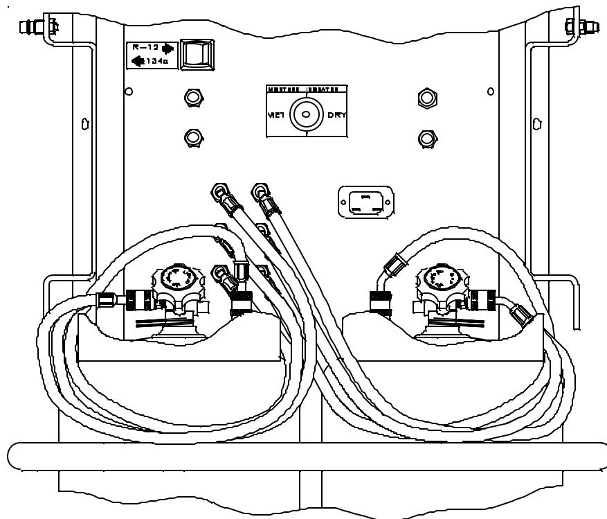
Diagram of Tank Installation
