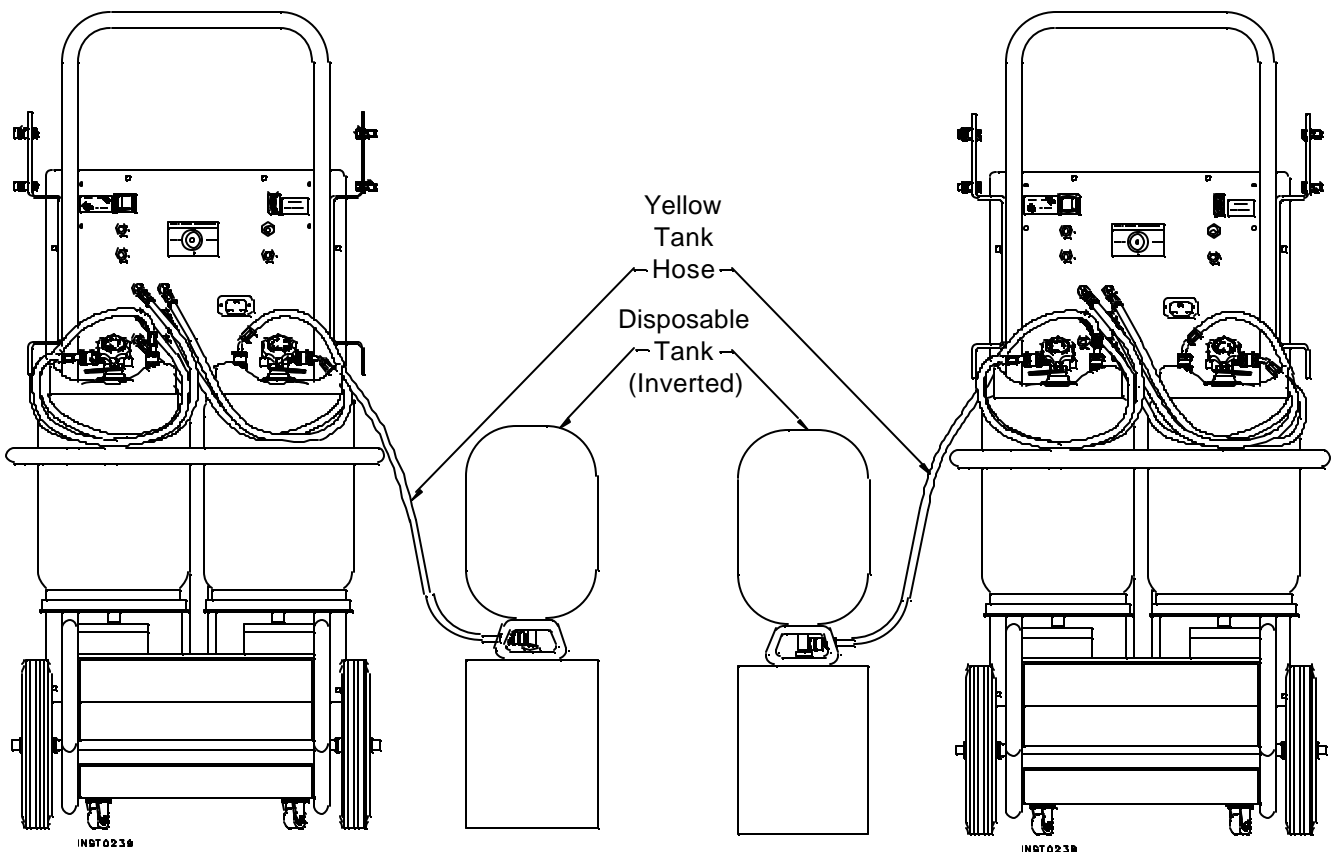
Diagram of Tank Connections When Partially Filling a Tank
